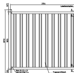
Transport and storage racks (for 25, 29 or 30 Tempofor panels and associated blocks – designed to be lifted using a forklift truck or a crane)
